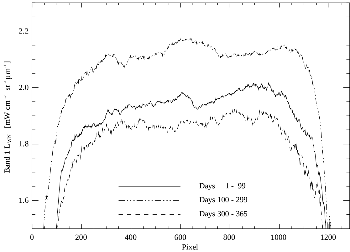
Fig. 21. The seasonal means of L_{WN} values as a function of pixel number along the scan line.
