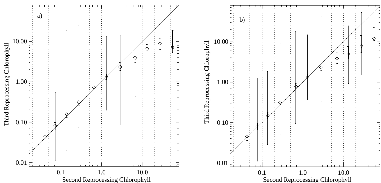
Fig. 8. Comparison of the chlorophyll retrieved in the third reprocessing ( y -axis) to that retrieved in the second reprocessing ( x -axis) for: a) 17–24 January 1998, and b) 12–19 July 1998. For level-3 binned chlorophyll a concentration from the second reprocessing in 11 ranges from 0.02–64.0 mg m -3 , the median third reprocessing chlorophyll value is plotted as diamonds. The nearest set of bars is the range of data in the second-to-third quartiles, while the outer bars show the extreme range of the third reprocessing chlorophyll values. Chlorophyll values greater than 2 mg m -3 were significantly reduced in the third reprocessing.
