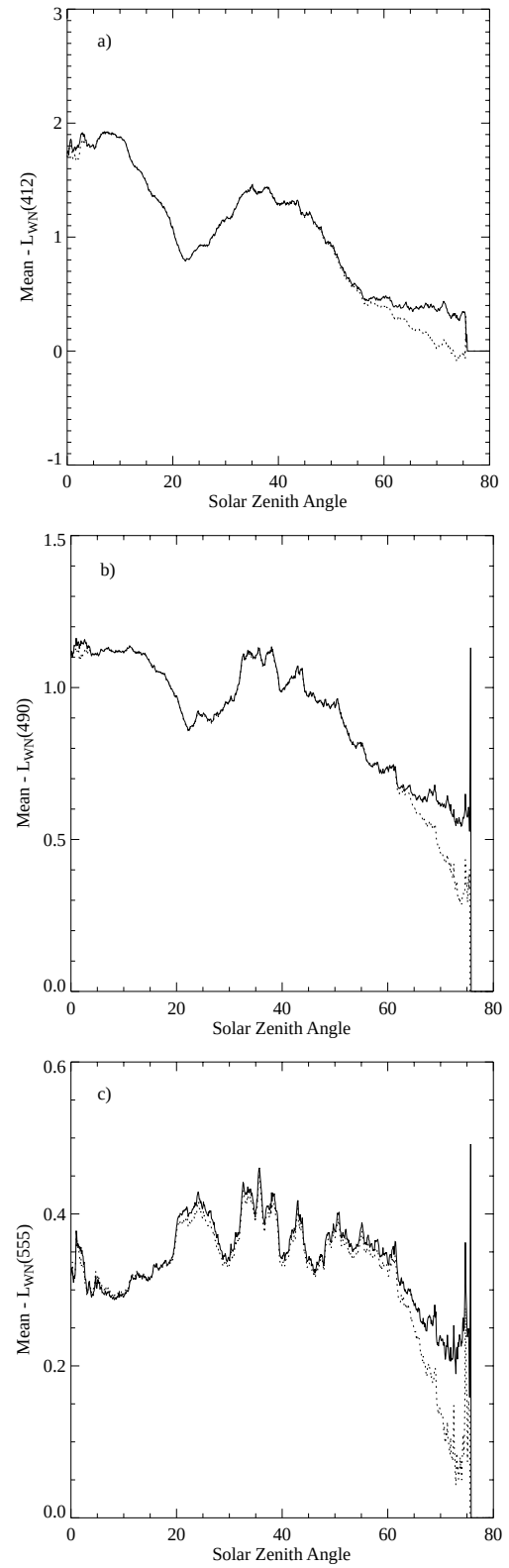
Fig. 11. Mean L_{WN} values as a function of solar zenith angle for the eight-day period of 12–19 July 1998 for the second (dotted curves) and third (solid curves) reprocessings. The SeaWiFS bands at a) 412, b) 490, and c) 555 nm are shown.
