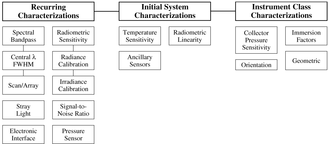
Fig. 1. Elements of radiometer characterization and calibration.
