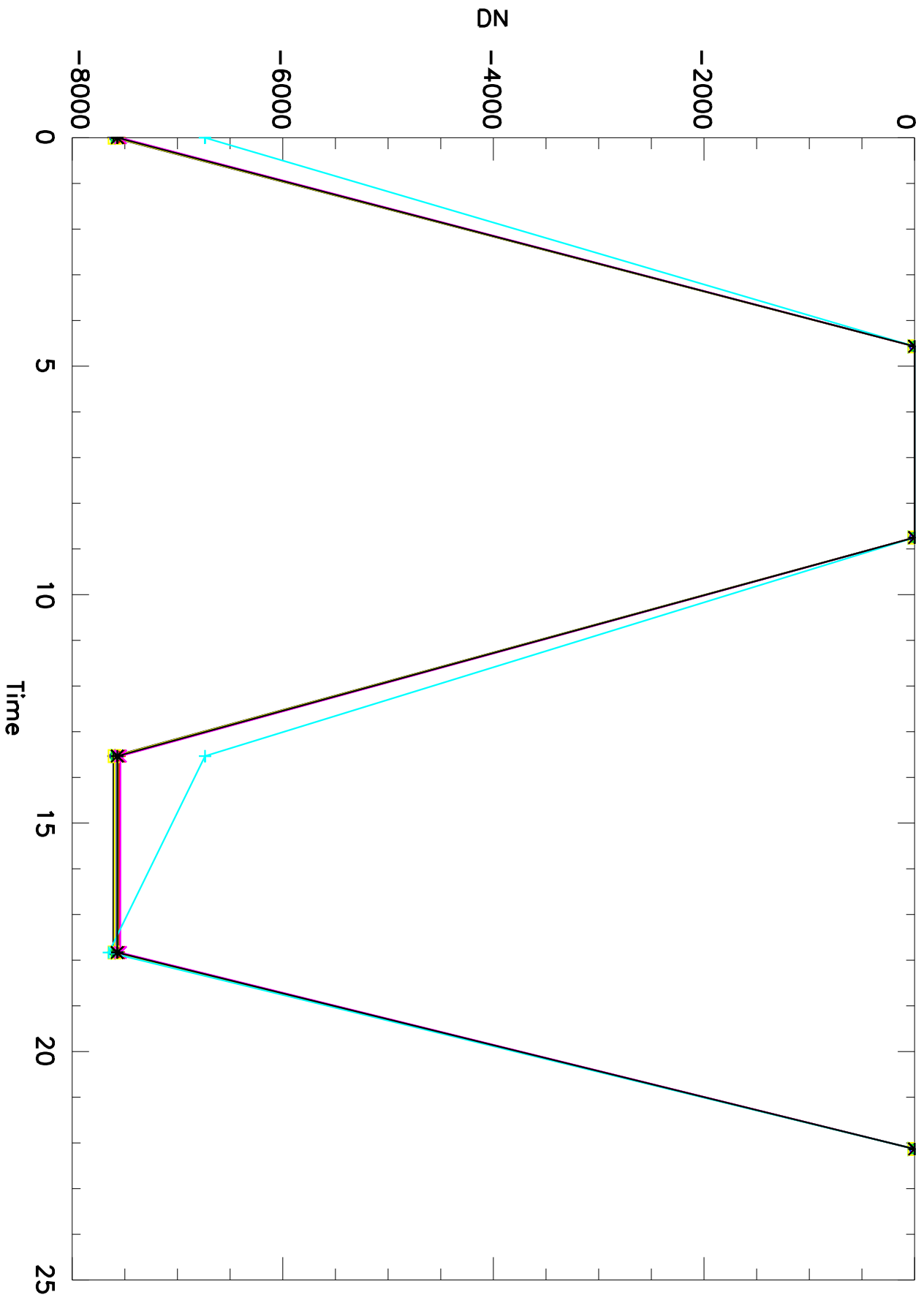
SDSM DN vs Time (SDSM SD)
