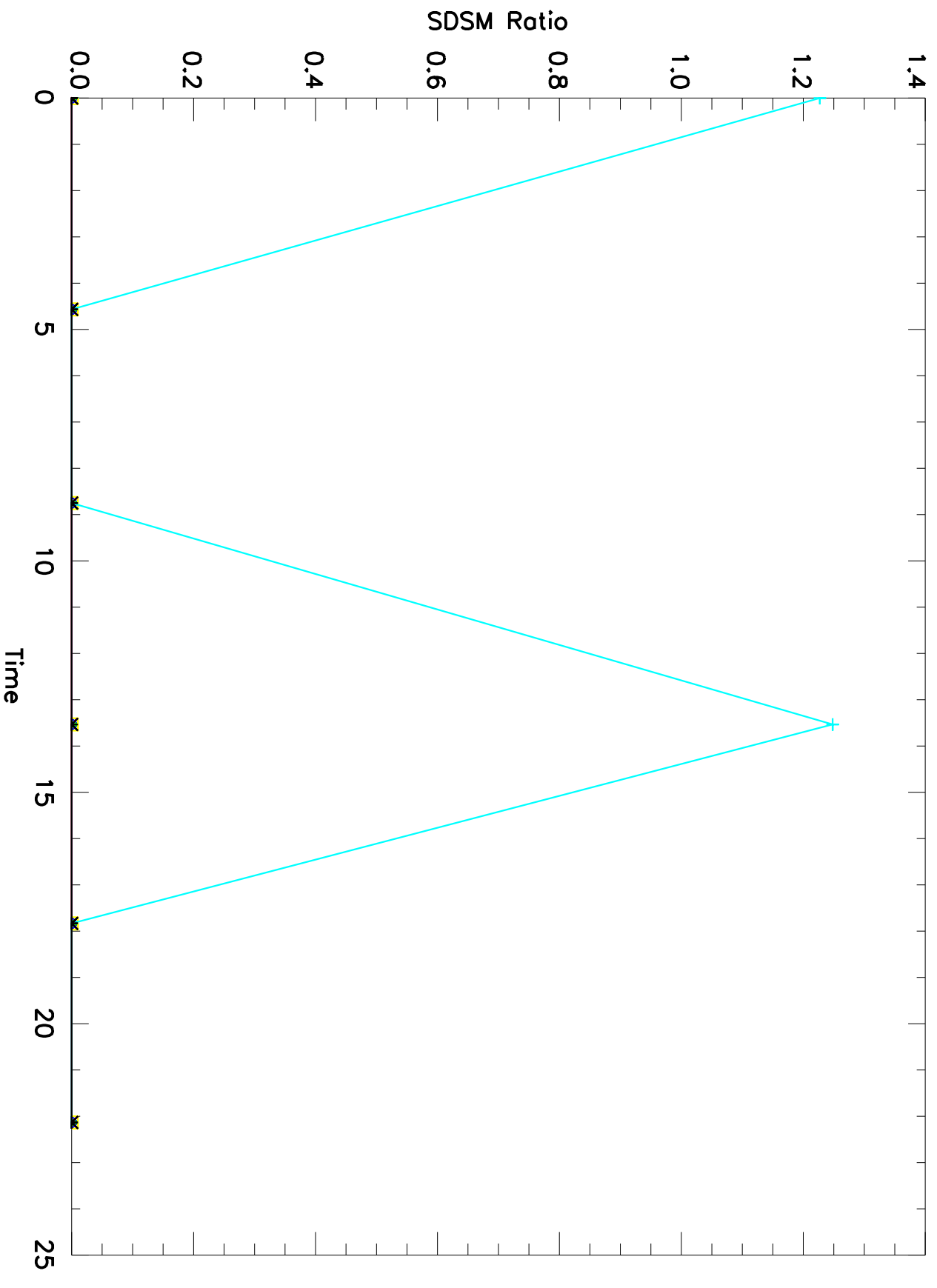
SDSM Ratio ( SD/Solar ) vs Time
