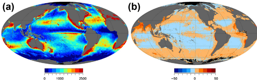
FIGURE 6 (a) Total number of match-ups between MODIS and SeaWiFS (2003–2007) on a 3rd-degree grid and (b) Mean relative difference \psi^* between SeaWiFS and MODIS (in %).
