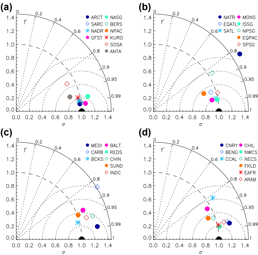
FIGURE 10 Taylor plots comparing SeaWiFS (taken as a reference) and MODIS-Aqua Chla time series averaged over biogeographic provinces associated with (a) midlatitudes, (b) subtropical regions, (c) marginal seas, and (d) shelves and upwelling regions. See Longhurst [84] for province acronyms.
