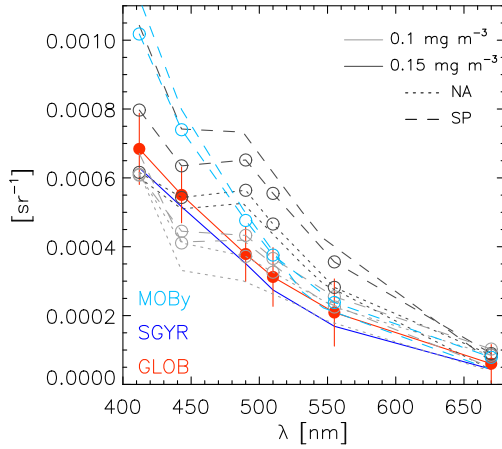
FIGURE 7 Uncertainty estimate \sigma obtained by collocation between SeaWiFS and MODIS, with global average (red) with standard deviation, and average over the subtropical gyres (blue). In gray are overplotted estimates of the uncertainty term proposed in [53] for SeaWiFS and MODIS as a function of Chl a for the North Atlantic (NA) and South Pacific (SP) subtropical gyres. Validation results \Delta_u obtained with Marine Optical Buoy (MOBy) data are shown in light blue. Curves with circles are for SeaWiFS.
