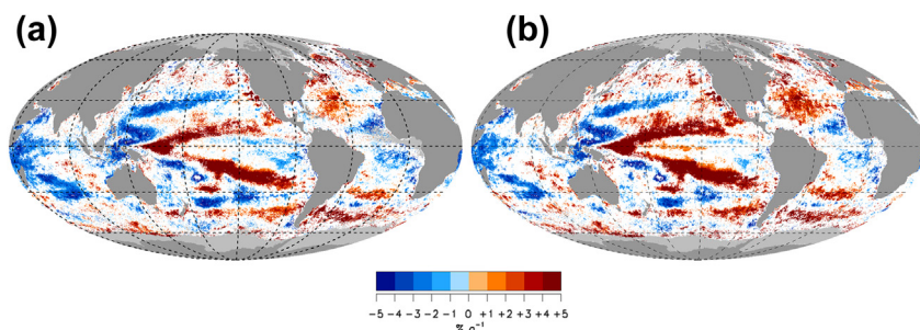
FIGURE 11 Linear trend for Chla (in % per annum) found over the period August 2002 to July 2011 for (a) MODIS-Aqua and (b) MERIS.
