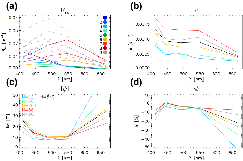
FIGURE 4 Dependence of validation statistics on optical water types at Acqua Alta Oceanographic Tower (AAOT). (a) Mean R_{rs} for the optical water types defined in [35]; type 9 includes eight subtypes. Validation results computed by types for (b) RMS difference \Delta , (c) mean absolute relative difference |\psi| , and (d) mean relative difference \psi . Results for all match-ups combined are in black; results per optical type are shown with the same color code as for (a) only if the members number at least 10 spectra.
