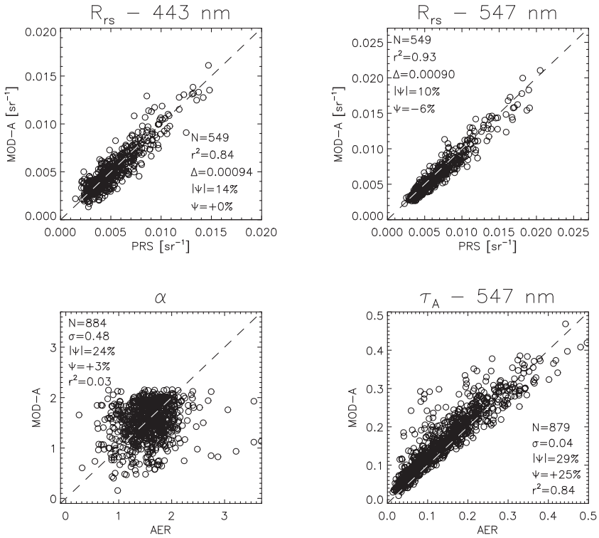
FIGURE 1 Comparison between above-water radiometry and MODIS-Aqua products for R_{rs} at 443 and 547 nm, and aerosol optical thickness \tau_A at 547 nm and Ångström exponent \alpha . Validation statistics are introduced in Section 2.2.
