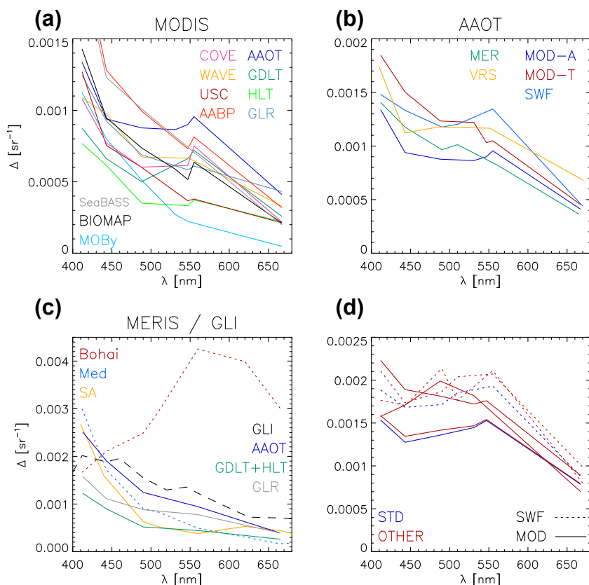
FIGURE 3 RMS differences between satellite and field data of R_{rs} (in \text{sr}^{-1} ): (a) MODIS-Aqua compared to various data sets from AERONET-OC sites (see text) as well as SeaWiFS Bio-optical Archive and Storage System (SeaBASS), BiOMaP, and Marine Optical Buoy (MOBy); (b) results for MODIS-Aqua ( N = 549 ) and Terra ( N = 270 ), MERIS ( N = 149 ), SeaWiFS ( N = 369 ) and VIIRS ( N = 70 ) at Acqua Alta Oceanographic Tower (AAOT); (c) results for MERIS processed by ESA processor (MERIS Ground Segment, MEGS, version 7 as dotted line, version 8 otherwise) given for the Bohai Sea [12], the northwest Mediterranean Sea [13], South African (SA) coastal waters [14], and AERONET-OC sites, AAOT ( N = 86 ), GDLT and HLT (Baltic Sea) and GLR (Black Sea) [15]. GLI results are represented by the black dashed line [16]. (d) Results obtained in coastal waters for SeaWiFS (dotted line) [17] and MODIS-Aqua [18] with different atmospheric correction schemes, including the standard SeaDAS (STD, in blue). When appropriate the reference source is given.
