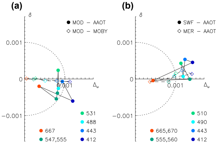
FIGURE 2 Spectral target diagram for validation results for MODIS-Aqua (a) at Marine Optical Buoy (MOBY) ( N = 229 ) and Acqua Alta Oceanographic Tower (AAOT) ( N = 549 , except at 531 nm, N = 176 ) and (b) SeaWiFS ( N = 369 ) and MERIS ( N = 149 ) at AAOT (right). Axes are in units of \text{sr}^{-1} . See text for the definition of statistical quantities.
