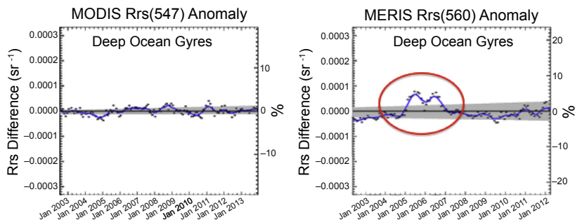
FIGURE 9 R_{rs} anomaly analysis for a global clear water region.
