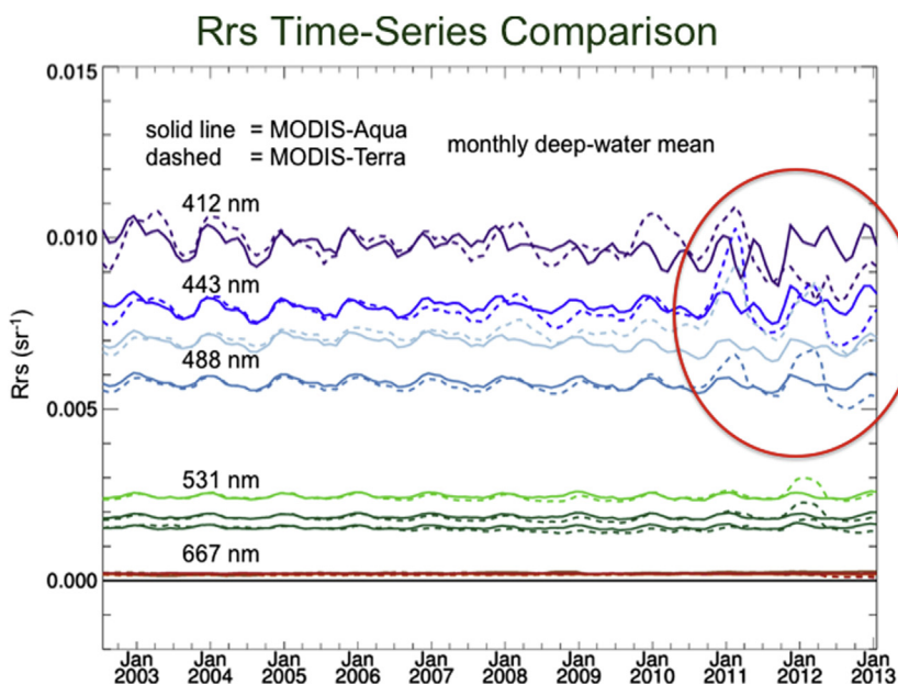
FIGURE 8 Comparative common-bin time-series of MODIS-Terra and MODIS-Aqua.
