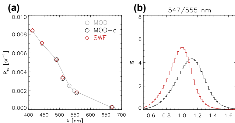
FIGURE 5 (a) Average of all daily R_{rs} coincident between MODIS-Aqua and SeaWiFS in 2003. Curve with gray circles represent MODIS values without band shifting, while black circles represent MODIS statistics computed after the band shifting correction has been applied. (b) Histogram of the ratio between MODIS (with and without band shifting, in red and black, respectively) and SeaWiFS R_{rs} in the green band.
