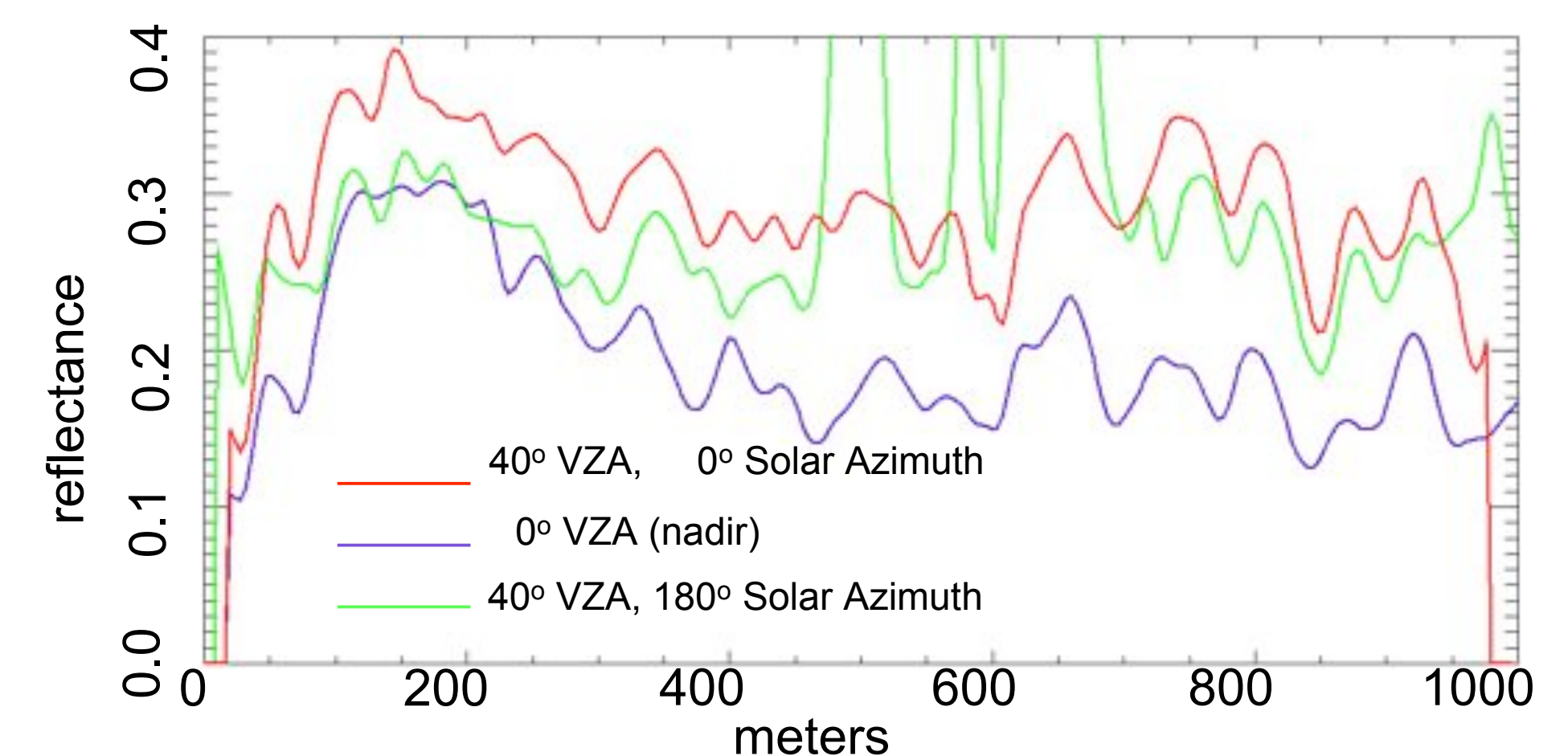
FIGURE 3 - Shown are NIR measurements made at three viewing angles along the transect during 4 Sept 2007.
