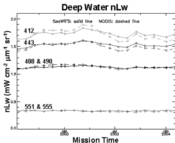
Figure 2b: Comparison of SeaWiFS Reprocessing 4 (solid line) and MODIS-Aqua (dashed line) normalized water-leaving radiance trends with MODIS-Aqua (dashed line) after initial OBPG reprocessing of MODIS using a common software and calibration approach.
