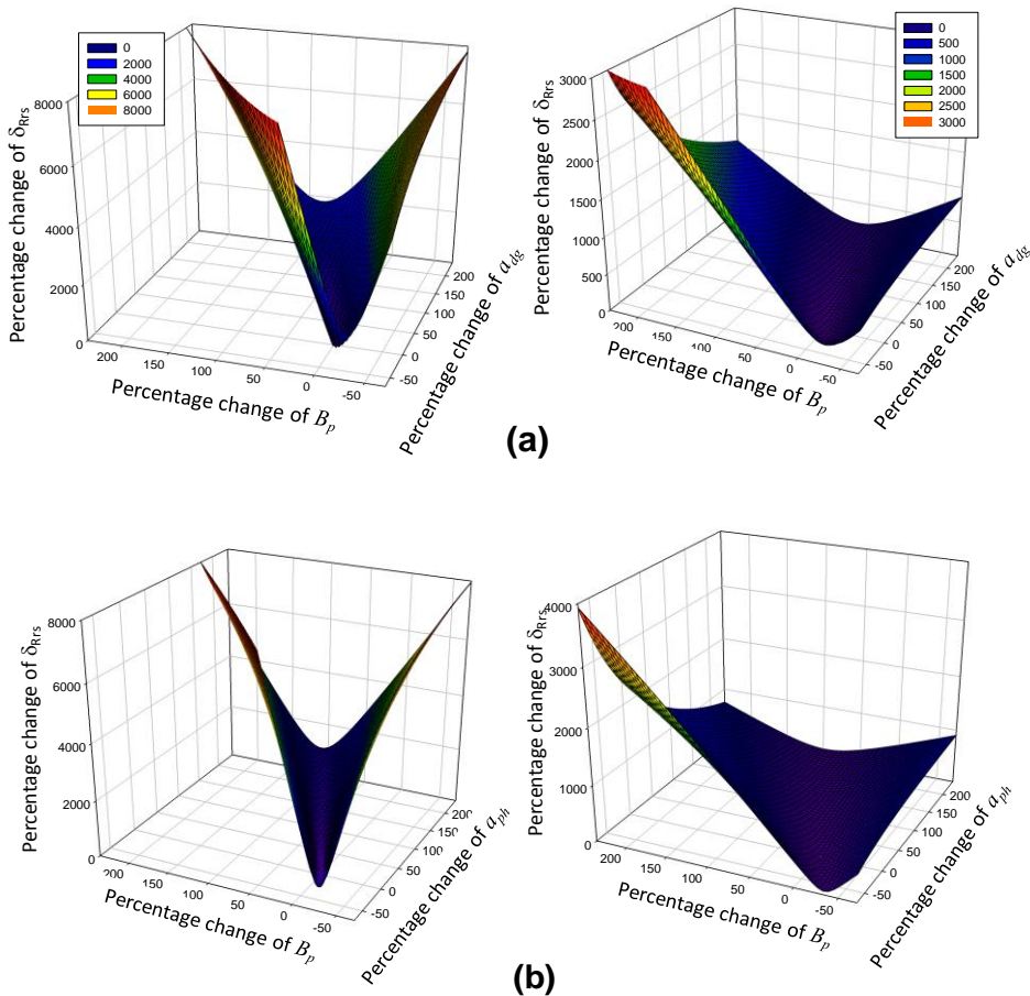
Figure 4. (a) Examples of surface shape of \delta_{Rrs} resulted from change of B_p and a_{dg} . (left) HOPE; (right) GSM; (b) Examples of surface shape of \delta_{Rrs} resulted from change of B_p and a_{ph} . (left) HOPE; (right) GSM.
